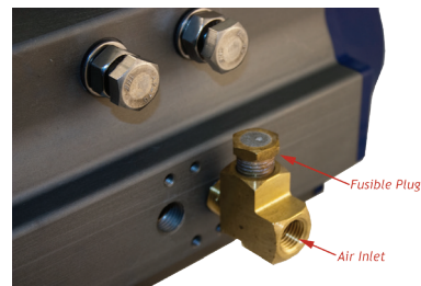
FUSIBLE PLUGS
